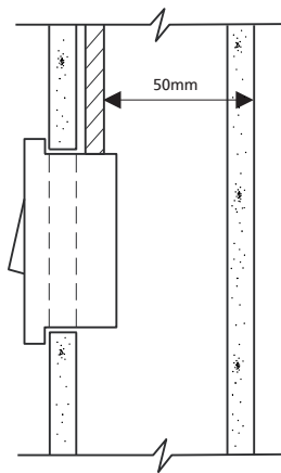
5 Minimum distance of cabling
