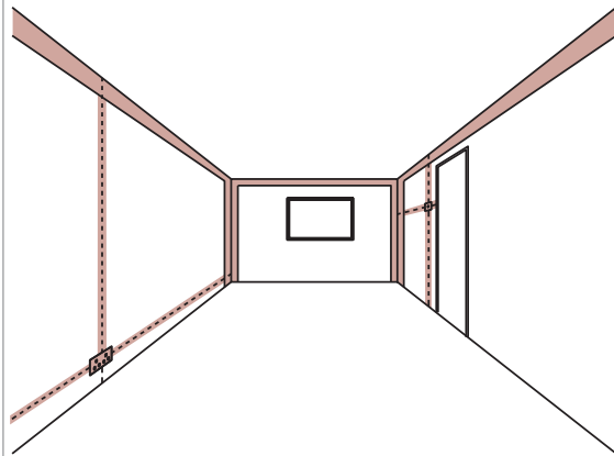
6 Standard zones of cabling
