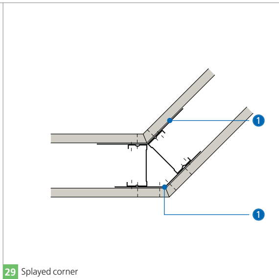
1 Gypframe GA6 Splayed Angle
