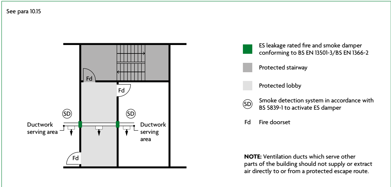
Diagram 10.3 Ductwork passing through protected escape routes – method 4
