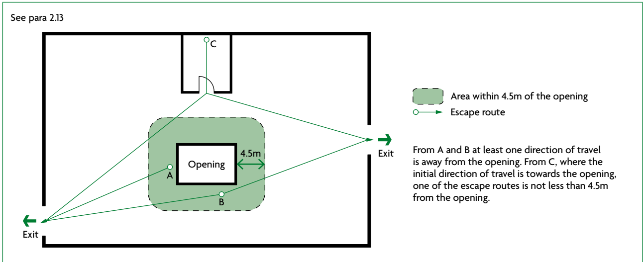
Diagram 2.5 Open connections
