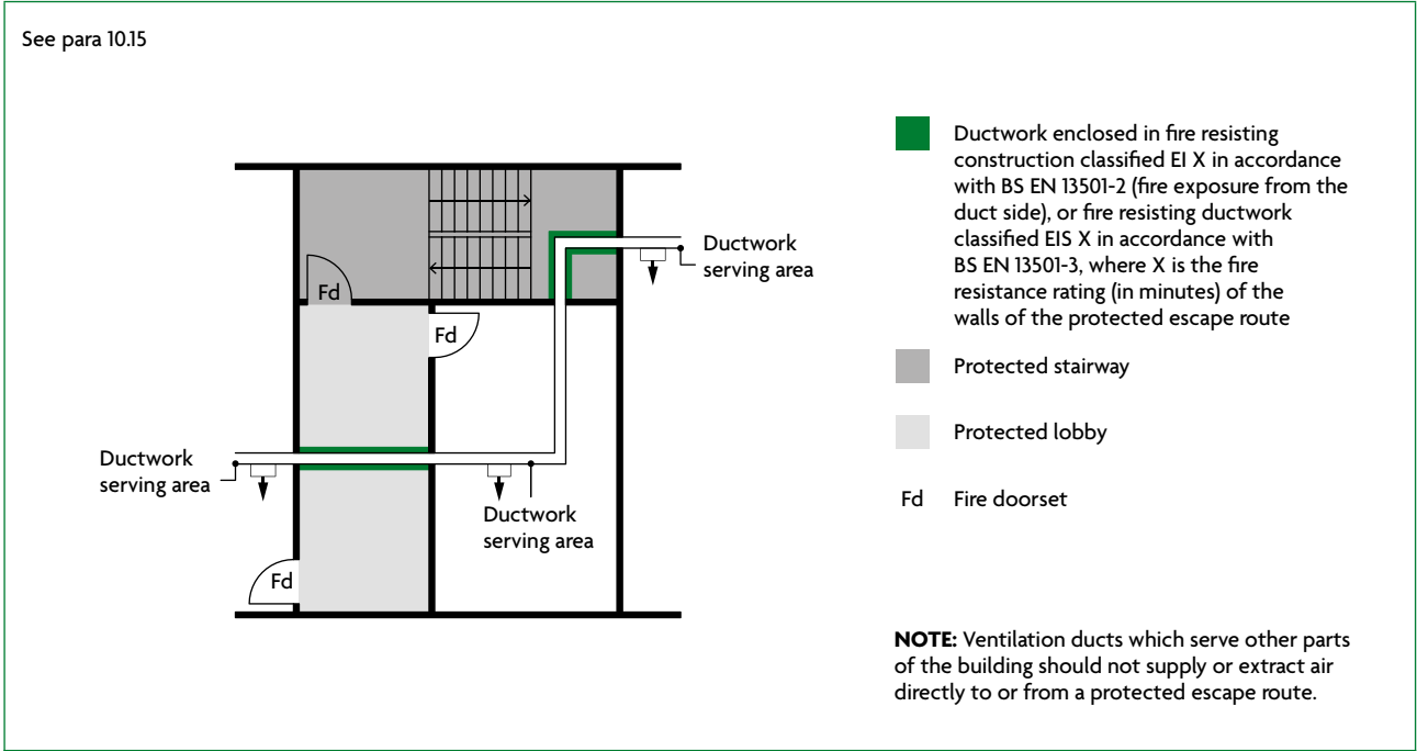
Diagram 10.2 Ductwork passing through protected escape routes – method 2 or method 3
