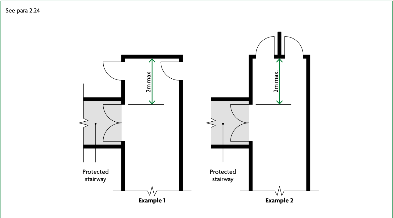
Diagram 2.8 Extension of corridor beyond a protected stairway
