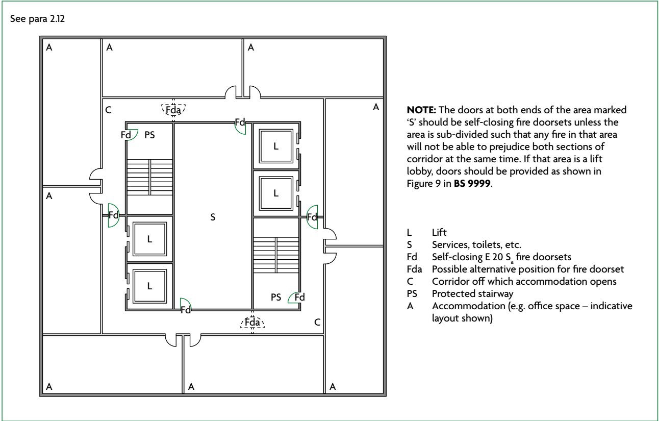
Diagram 2.4 Exits in a central core
