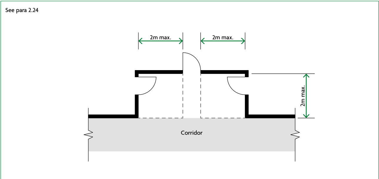
Diagram 2.7 Recesses off corridors
